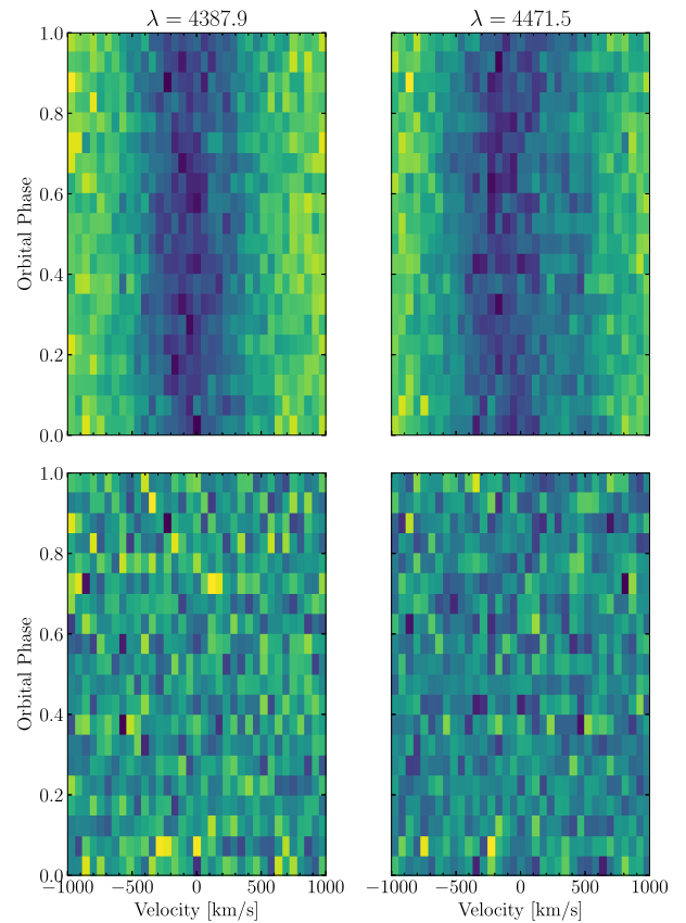
Figure 12. Top row: Trailed spectra of TIC 378898110 from 2021 July 05, created using 49 back-to-back, one-minute exposures with Goodman + SOAR, phase-folded on the 23.07 min period and showing the 4387.9 and 4471.5 Å He I lines (left and right, respectively). Bottom row: The same trailed spectra with the mean spectrum (Fig. 10) subtracted from each. We do not see any periodic feature in the residuals.
