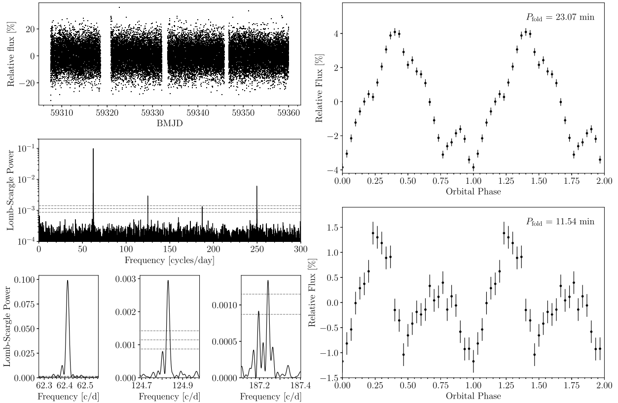
Figure 1. Top left: TESS light curve from Sectors 37 and 38, showing flux change relative to the mean. Middle left: Lomb-Scargle periodogram of the TESS light curve. Dashed horizontal lines show false alarm probabilities of 0.1, 10^{-3} , and 10^{-5} . Lower left: Zoomed plots of the periodogram peaks around the 23.07 min period and its first two harmonics, with the same false alarm probabilities marked (c/d refers to cycles per day). Note the change in y-axis scale from logarithmic to linear. Top right: Phase-folded and binned TESS light curve, folded on the 23.07 min period. Lower right: Phase-folded and binned TESS light curve, folded on the first harmonic at 11.5 min.
