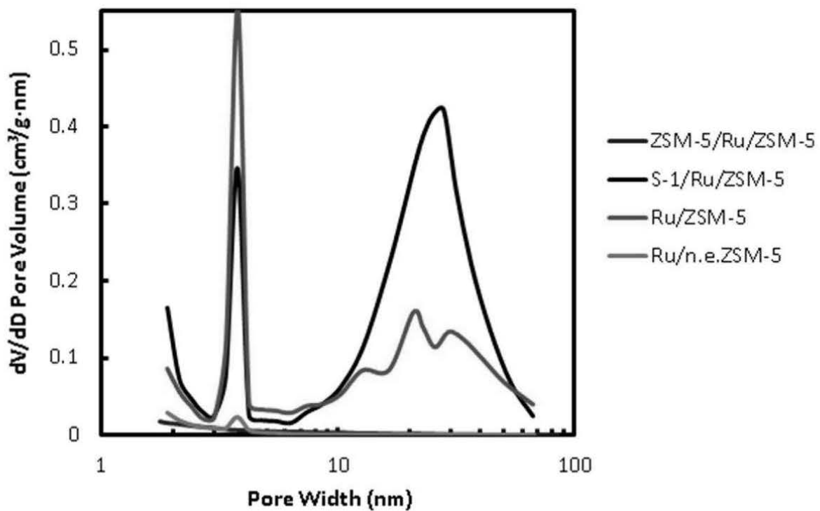
Figure S7: BJH pore size distribution curves for Ru zeolite nanocomposite catalysts.
