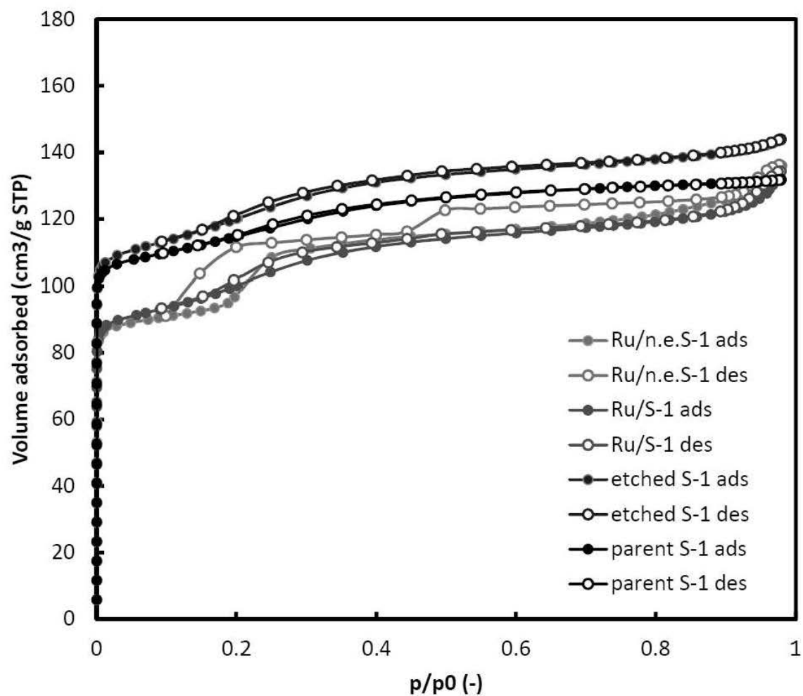
Figure S6: N 2 sorption isotherms for parent and fluoride-etched S-1 compared with corresponding Ru/n.e.S-1 and Ru/S-1 catalysts; note that the low pressure hysteresis is truly more pronounced for the Ru/n.e.S-1 than for Ru/S-1 although one would expect it vice versa; empty points denote desorption (n.e. nonetched).
