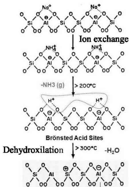
Figure 1.3. Formation of Brønsted acid sites and transformation in Lewis acid sites.
