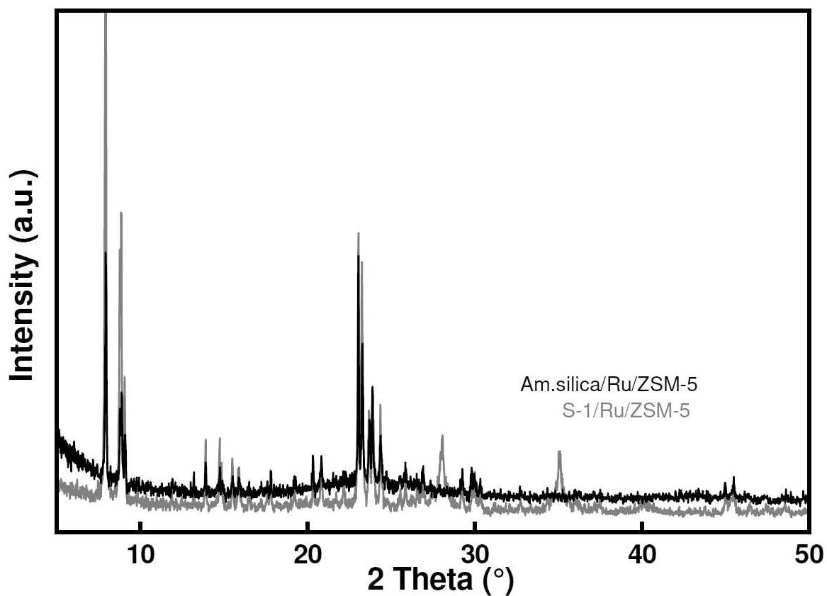
Figure S3: Powder XRD patterns of S-1/Ru/ZSM-5 catalyst (gray) vs. a composite Am. silica/Ru/ZSM-5 having an amorphous shell; note the baseline elevation between 2\theta = 20^\circ and 30^\circ documenting the presence of amorphous silica phase.
