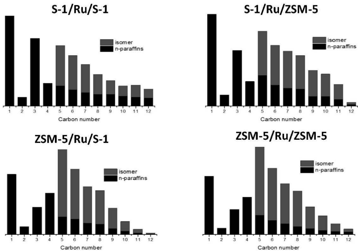
Figure S10: Hydrocarbon distribution graphs observed over coated catalysts.
