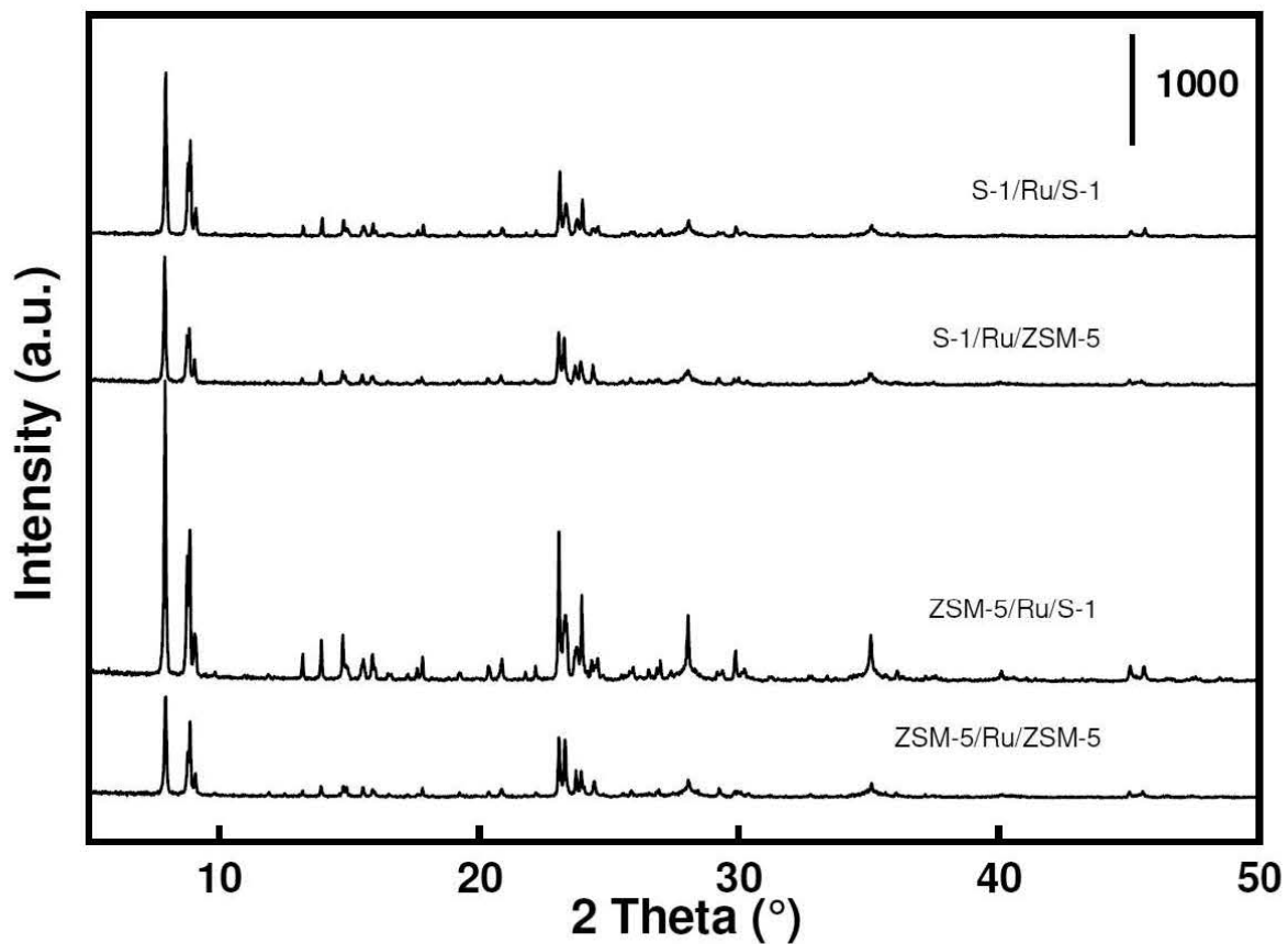
Figure S1: Powder XRD patterns of the final catalysts with zeolitic shells prepared by coating the parent MFI crystals after insertion of Ru nanoparticles; catalysts are after calcination and ionexchange; the reduction was performed in-situ when charged into the reactor.
