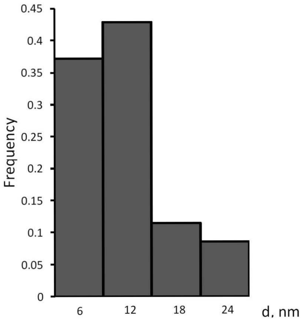
Figure S4: Histogram of ruthenium particle size distribution in Ru/ZSM-5.
