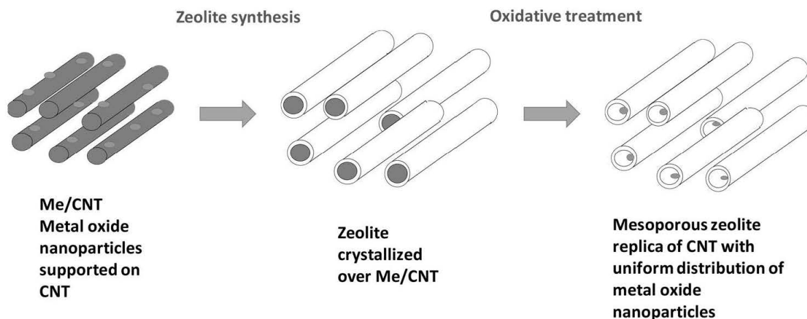
Figure 1.9. Synthesis of metal-zeolite nanocomposites using metal/CNT as secondary hard templates [52].
