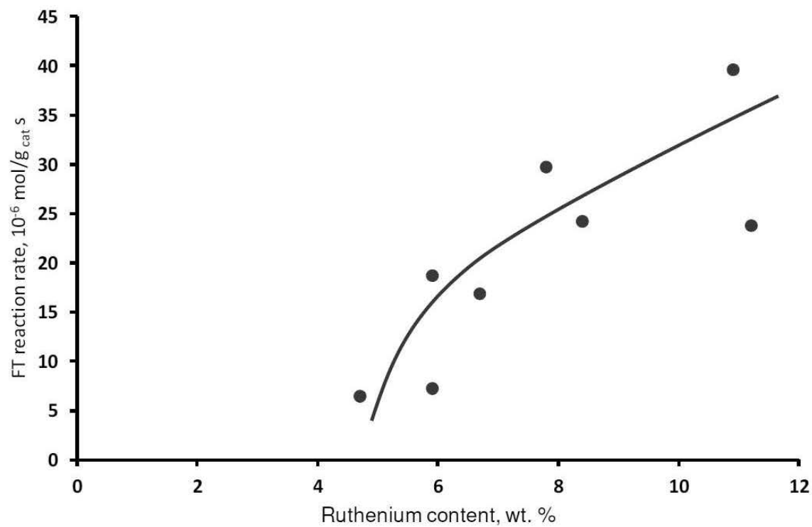
Figure S9. FT reaction rate versus Ru content in the Ru-zeolite nanocomposite catalysts.
