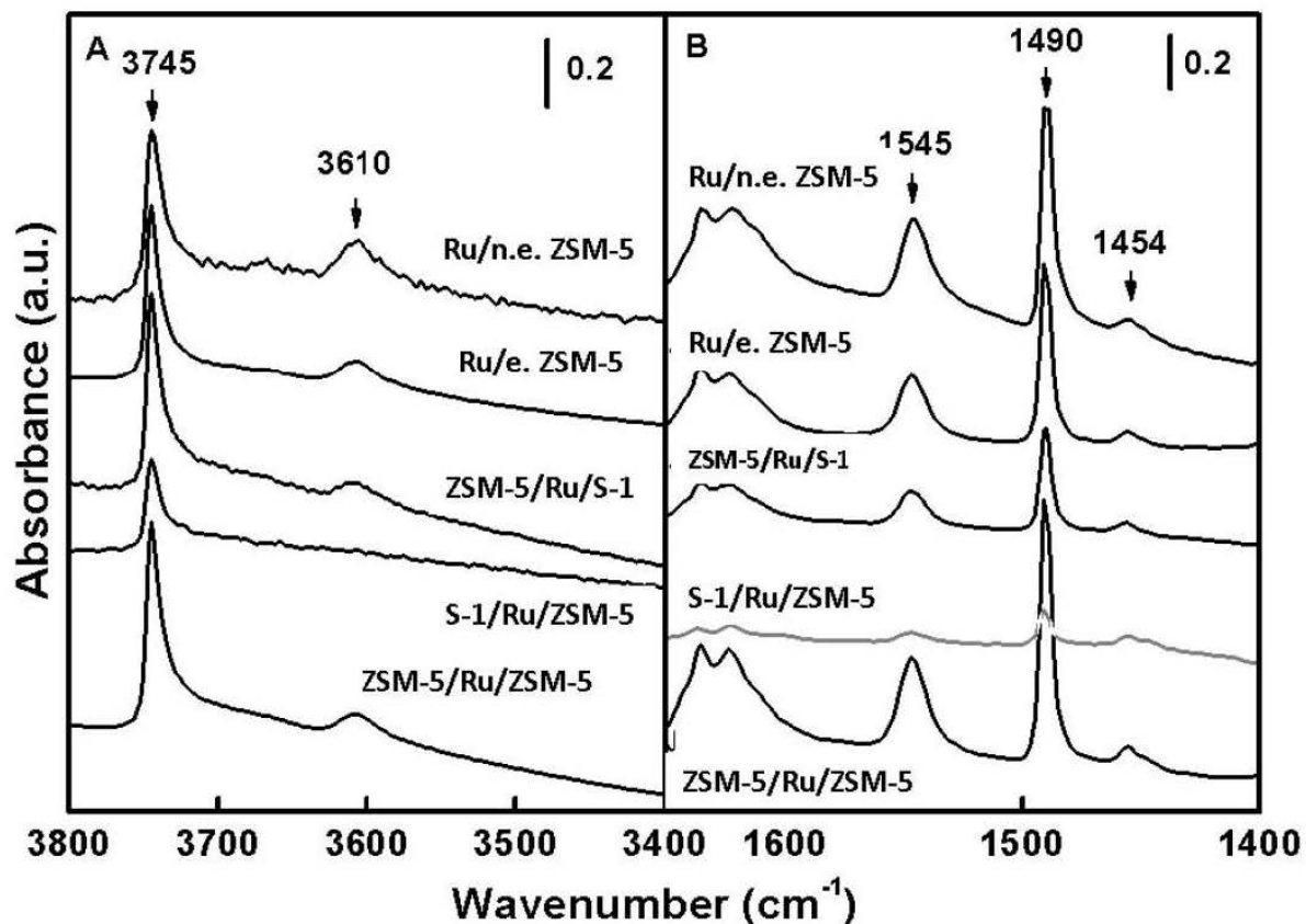
Figure S5: IR spectra of the metal-zeolite catalysts. A: -OH region after activation at 450°C; B: region of pyridinium vibrations after pyridine adsorption and desorption at 150°C for 15 min. Note that the signal of terminal silanol groups at 3745 cm -1 is influenced by the presence of fumed silica used to dilute the sample to maintain sufficient pellet transparency (n.e. nonetched).
