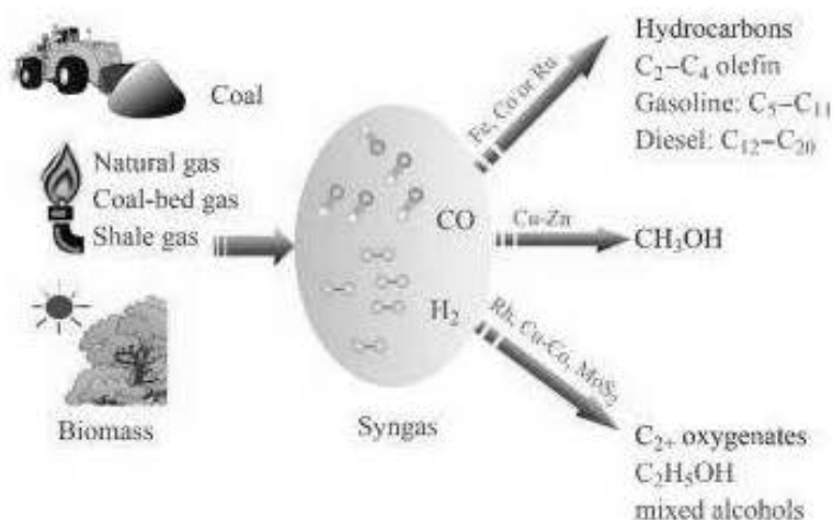
Figure 1.10. Conversion of non-petroleum sources into liquid fuels and chemicals via syngas [61].
