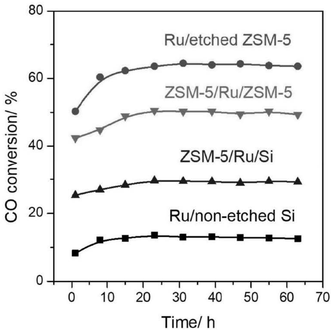
Figure S8: Carbon monoxide conversion as a function of time on stream over ruthenium-zeolite catalysts. Conditions: GHSV=6502 cm 3 /g.h, H 2 /CO=2, P=20bar, T=250 °C.
