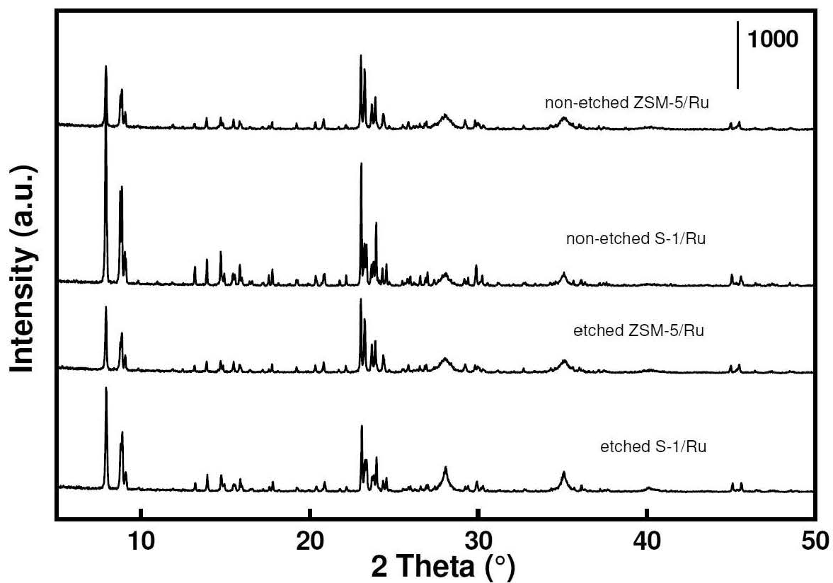
Figure S2: Powder XRD patterns of the final catalysts without the coating shell; catalysts are after calcination and ion-exchange; the reduction was performed in-situ when charged into the reactor.
