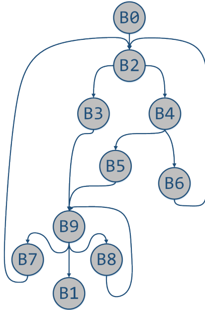
Figure 3.4: Example control-flow graph partitioning of a program.
