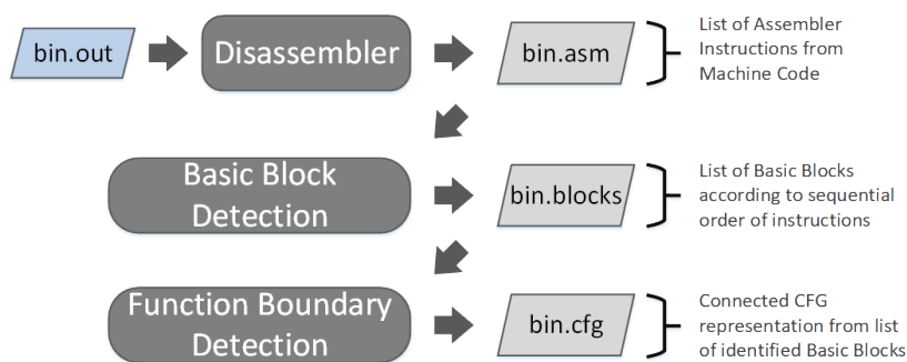
Figure 5.7: CFG generation process from the executable binary code.
