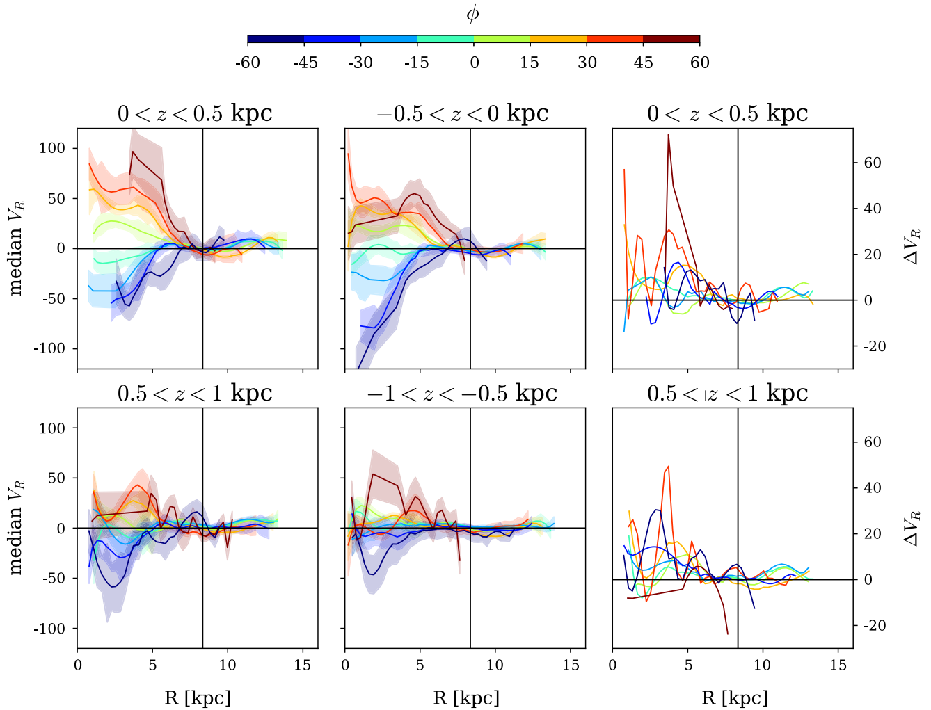
Figure 5. V_R as a function of R for different azimuth slices \phi and heights from the plane z . The error bars correspond to the standard error of the median. The black solid lines represent V_R = 0 \text{ km s}^{-1} and the solar position. The left and middle columns show the results obtained for the Northern and Southern hemisphere, respectively, while the right column shows the V_R residuals between both Galactic hemispheres. The striking feature is the systematic shift seen in the inner disc, smoothly changing from positive V_R at positive \phi to negative V_R at negative \phi .
