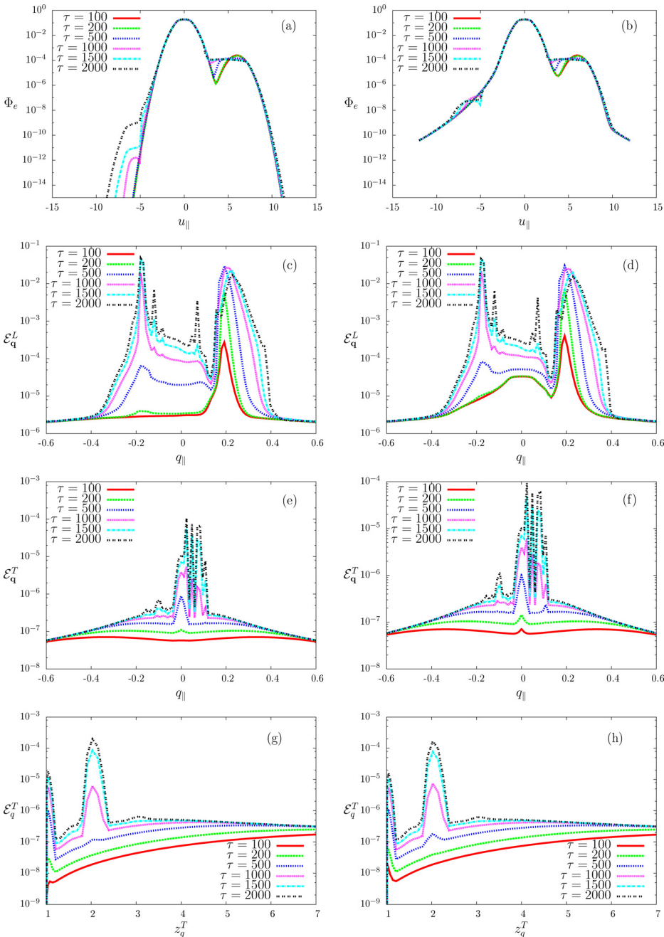
FIG. 5. (a) 1D electron distribution function vs. u_{\parallel} , for several values of \tau , for n_{\kappa e}/n_e=0.0 ; (b) 1D electron distribution function vs. u_{\parallel} , for several values of \tau , for n_{\kappa e}/n_e=5.0 \times 10^{-2} ; (c) 1D spectrum of L waves vs. q_{\parallel} , for several values of \tau , for n_{\kappa e}/n_e=0.0 ; (d) 1D spectrum of L waves vs. q_{\parallel} , for several values of \tau , for n_{\kappa e}/n_e=5.0 \times 10^{-2} ; (e) 1D spectrum of T waves vs. q_{\parallel} , for several values of \tau , for n_{\kappa e}/n_e=0.0 ; (f) 1D spectrum of T waves vs. q_{\parallel} , for several values of \tau , for n_{\kappa e}/n_e=5.0 \times 10^{-2} . (g) Spectrum of T waves vs. q , for several values of \tau , for n_{\kappa e}/n_e=0.0 . (h) Spectrum of T waves vs. q , for several values of \tau , for n_{\kappa e}/n_e=5.0 \times 10^{-2} . The parameters are the same as those used in Fig. 4.
