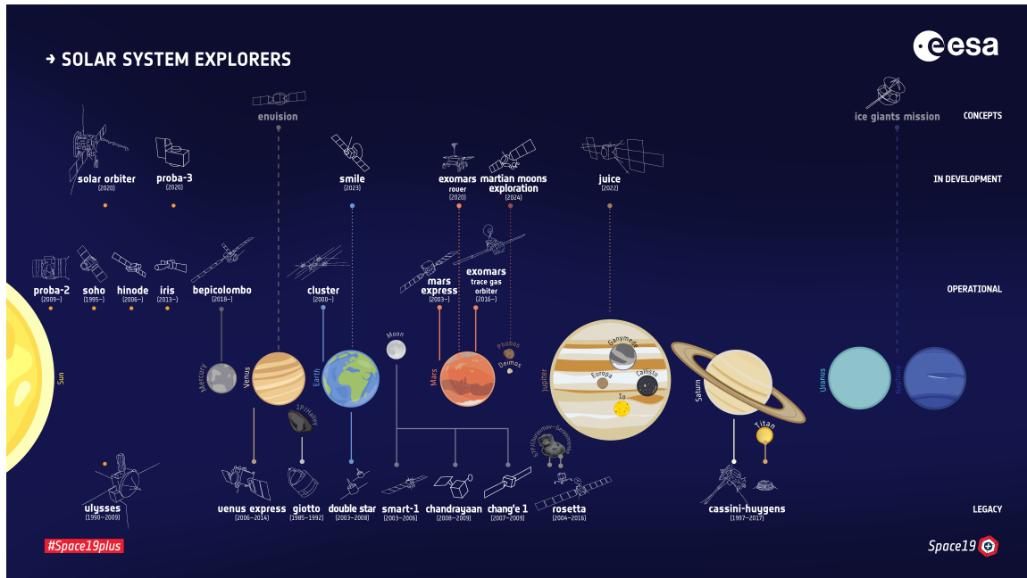
Figure 1.3: ESA’s past, present, and future science missions for studying the solar system.
