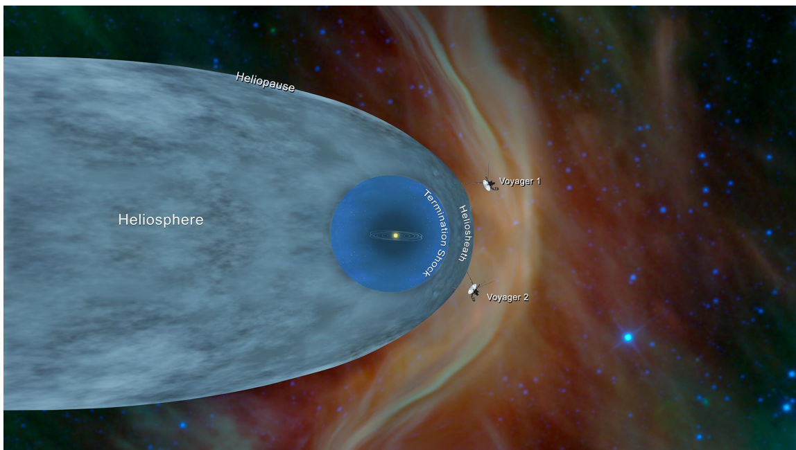
Figure 1.1: Main boundaries of the heliosphere and the location of both Voyager missions.
