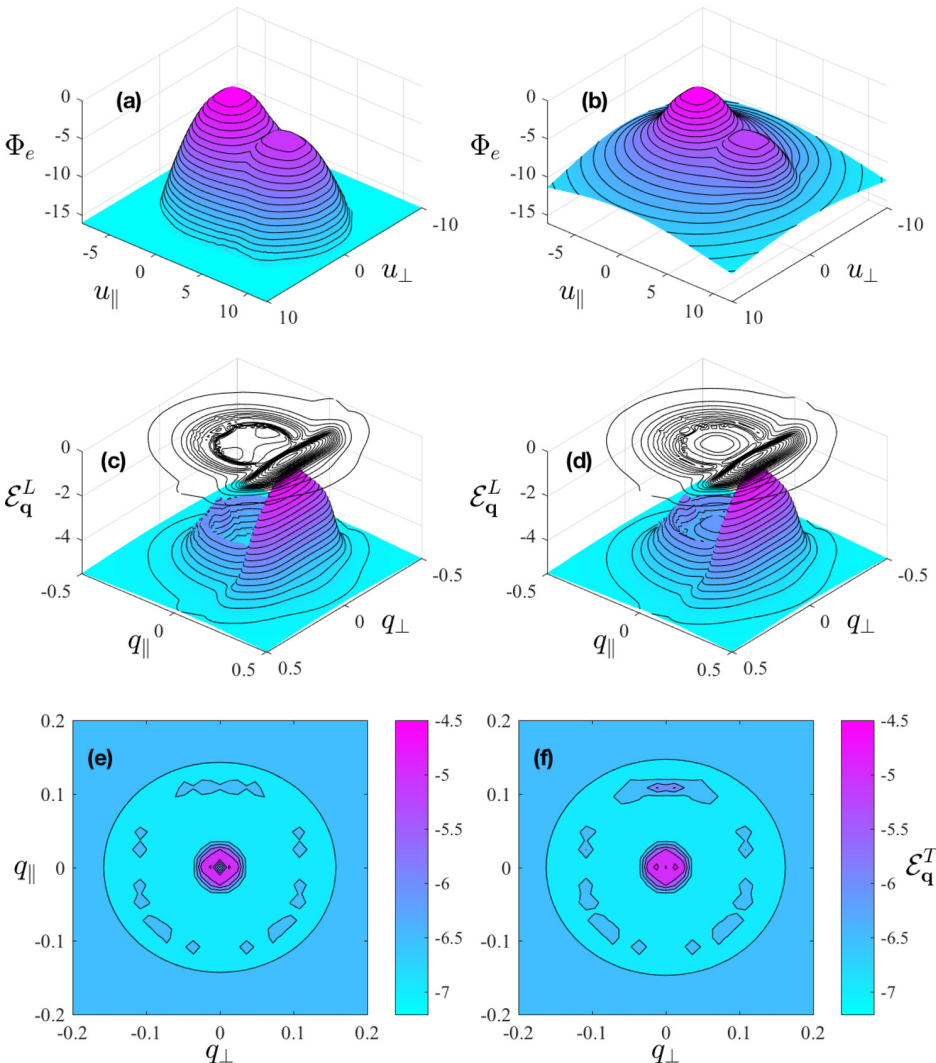
FIG. 4. (a) Electron distribution function at \tau = 500 , vs. u_{\parallel} and u_{\perp} , for n_{\kappa el}/n_e = 0.0 ; (b) electron distribution function at \tau = 500 , vs. u_{\parallel} and u_{\perp} , for n_{\kappa el}/n_e = 5.0 \times 10^{-2} ; (c) spectrum of L waves at \tau = 500 , vs. q_{\parallel} and q_{\perp} , for n_{\kappa el}/n_e = 0.0 ; (d) spectrum of L waves at \tau = 500 , vs. q_{\parallel} and q_{\perp} , for n_{\kappa el}/n_e = 5.0 \times 10^{-2} ; (e) spectrum of T waves at \tau = 500 , vs. q_{\parallel} and q_{\perp} , for n_{\kappa el}/n_e = 0.0 ; and (f) spectrum of T waves at \tau = 500 , vs. q_{\parallel} and q_{\perp} , for n_{\kappa el}/n_e = 5.0 \times 10^{-2} . Input parameters are as follows: T_e/T_i = 2.0 , T_b/T_e = 1.0 , n_b/n_e = 1.0 \times 10^{-3} , v_b/v_e = 6.0 , g = 5.0 \times 10^{-3} , and \kappa_e = 5.0 .
