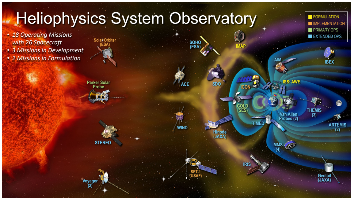
Figure 1.2: NASA’s present and future heliophysics system observatory. The number between parenthesis under the probe’s name is the total number of spacecrafts that compose the mission.
