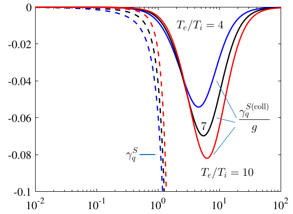
FIG. 2. Normalized collisional damping for S waves, \gamma_q^{S(coll)}/g , vs normalized wavenumber q , for three values of the ratio T_e/T_i .
