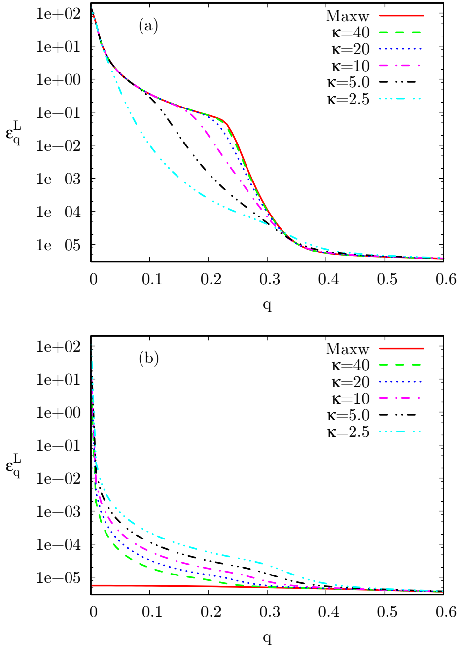
Figure B.1: Asymptotic spectrum of Langmuir waves for several values of \kappa index and Maxwellian distribution. (a) With electrostatic bremsstrahlung emission and collisional damping. (b) Without bremsstrahlung emission and collisional damping.
