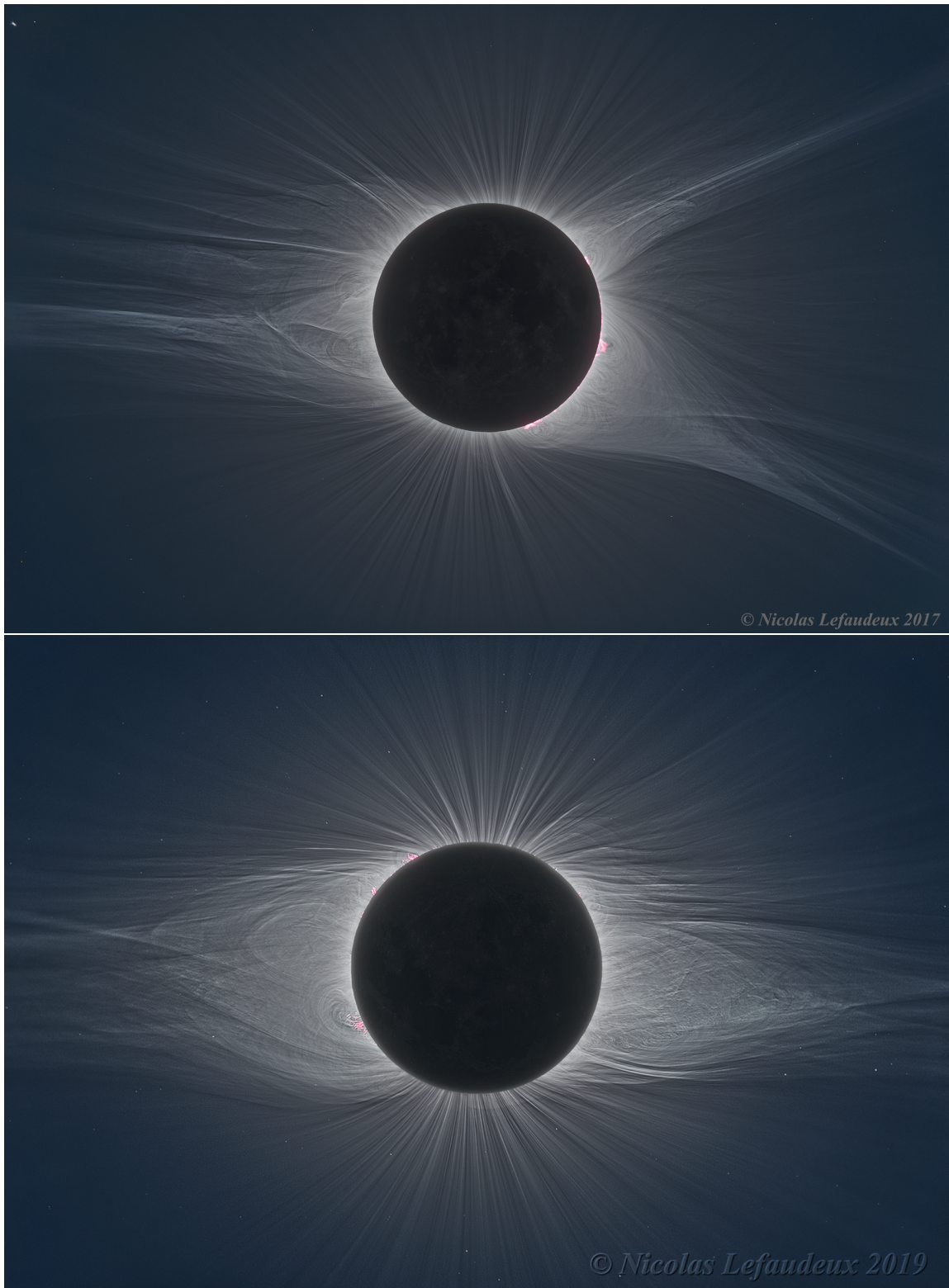
Figure 1.4: Solar corona captured during the total solar eclipse of 2017 (top panel) and 2019 (lower panel). The reddish contour at some regions is the chromosphere, and the reddish arcs are solar prominences, chromospheric plasma structures that penetrate the coronal region. Credit: Nicolas Lefaudeux , accessed at 15/08/2019.
