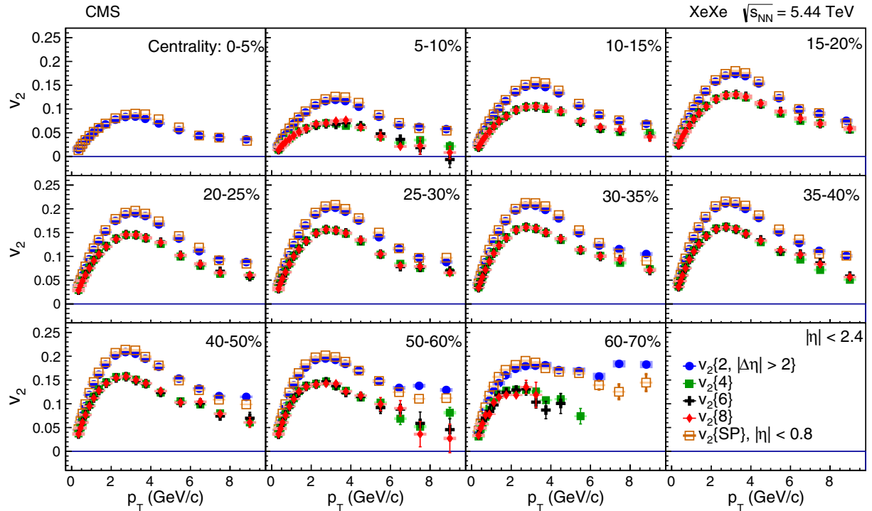
FIG. 1. Elliptic-flow coefficients v_2 based on different analysis techniques, as functions of transverse momentum and in bins of centrality, from the 5% most central (top left) to 60–70% centrality (bottom right). The results for the two-particle and multiparticle correlations correspond to the range |\eta| < 2.4 , while the scalar-product results are for |\eta| < 0.8 . The bars and the shaded boxes represent statistical and systematic uncertainties, respectively.
