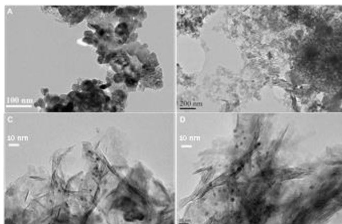
Figure 4-2 TEM images of Co (10-20) /ZSM-5 (A), CoCNT (10-20) /ZSM-5(B), CoCNT (10-20) /ZSM-5 high magnification(C) and CoCNT (20-40) /ZSM-5 high magnification.
