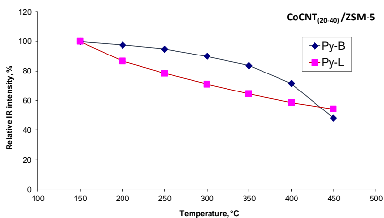
Figure S5. Variation of intensities of IR bands attributed to Pyridine adsorbed on Brönsted and Lewis acid sites as functions of desorption temperature on different cobalt-zeolite catalysts. The zeolites synthesized using CNT impregnated with cobalt have slightly stronger Brönsted acid sites compared to the samples prepared by impregnation.
