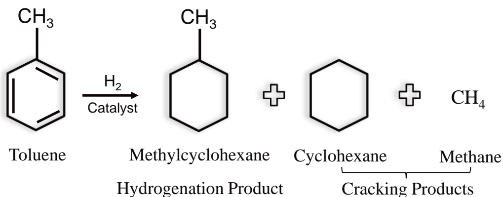
Figure 2-11 Toluene hydrogenation and products cracking [98] .
