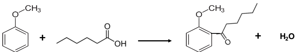
Figure 5-9 Acylation of anisole with hexanoic acid results in ortho-methoxy-hexyl-phenone.
