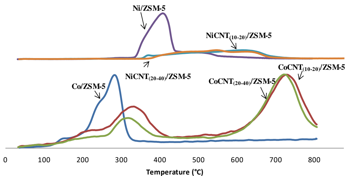
Figure 5-7 Temperature programmed reduction (TPR) profiles of the Co (a) and Ni (b) catalysts.
