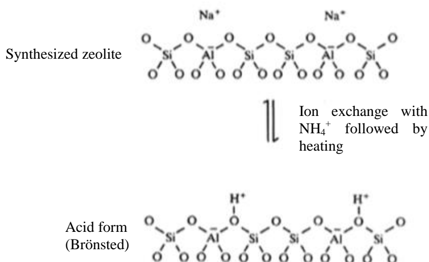
Figure 2-6 Formation of Brønsted acid sites in zeolites (adapted from [51]).
