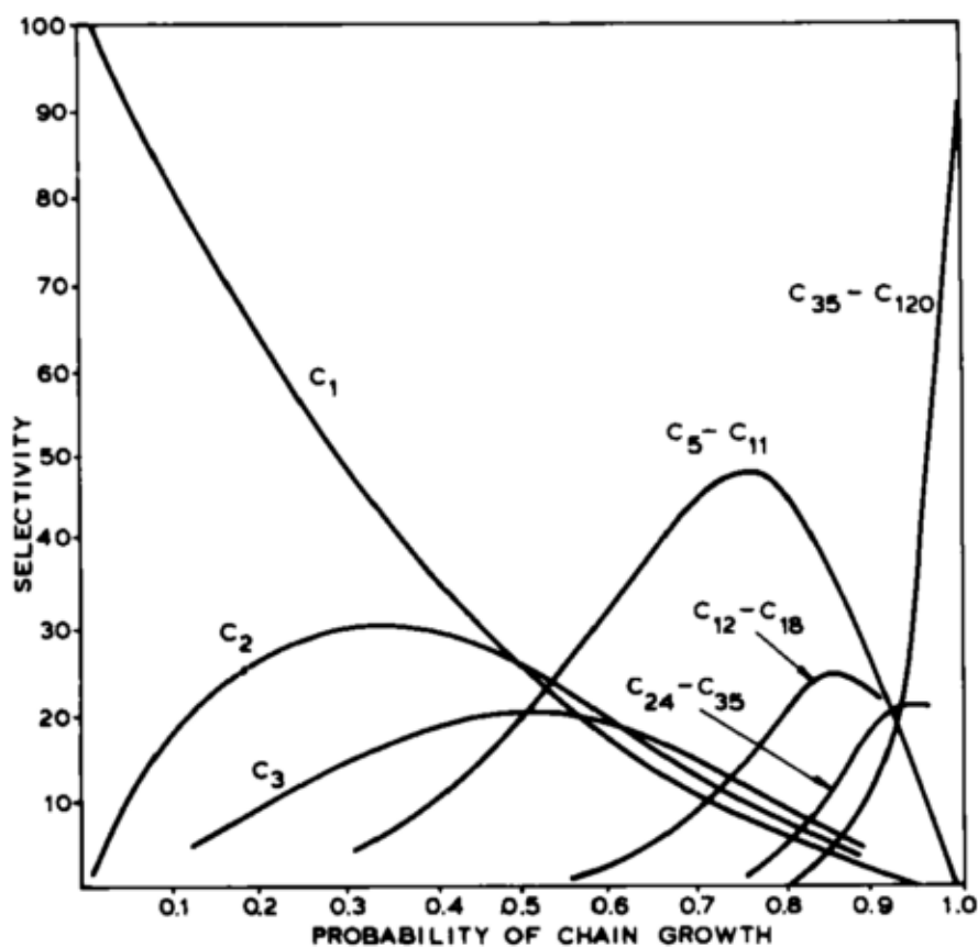
Figure 2-14 Hydrocarbons selectivity as \alpha function [108] .
