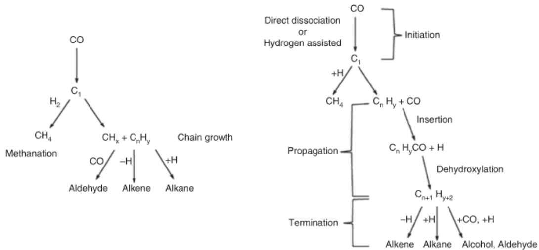
Figure 2-13 FTS mechanism [106] .
