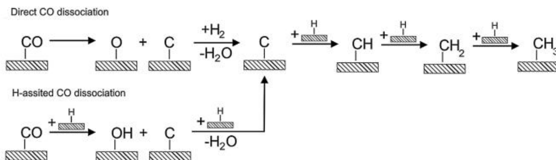
Figure 2-15 Carbene mechanism [113] .
