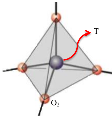
Figure 2-1 Zeolite structure adaptaded from [20] .
