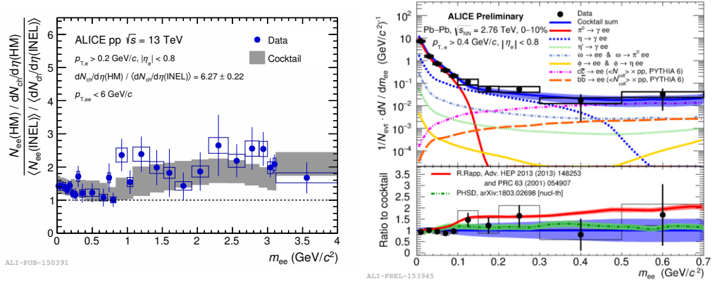
Fig. 3. Left panel: Ratio of dielectron spectra scaled with charged-particle multiplicity in inelastic and high-multiplicity pp collisions at \sqrt{s} = 13 TeV, compared to the expectations from hadronic sources. Right panel: dielectron invariant-mass spectrum in the 0-10% most central Pb-Pb collisions at \sqrt{s_{NN}} = 2.76 TeV compared to cocktails with and without thermal radiation from the medium [6, 7].
