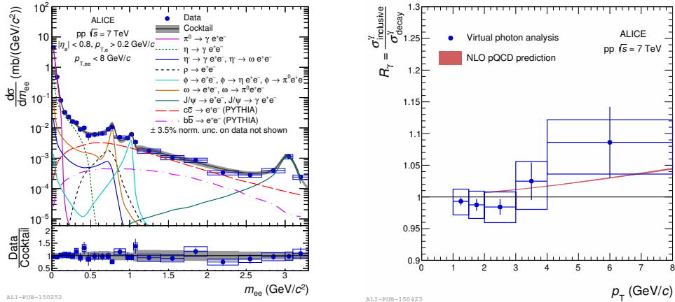
Fig. 1. Left panel: m_{ee} -differential e^+e^- cross section in pp collisions at \sqrt{s} = 7 \text{ TeV} for p_{T,e} > 0.2 \text{ GeV}/c and |\eta_e| < 0.8 compared with a cocktail of expected hadronic sources [1]. Right panel: ratio of inclusive-to-decay photon cross sections measured in pp collisions at \sqrt{s} = 7 \text{ TeV} compared to pQCD calculations [1, 4].
