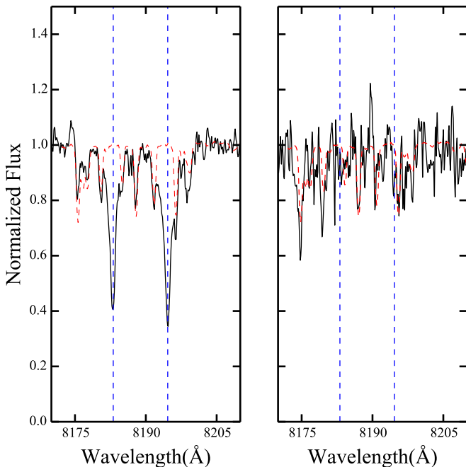
Figure 5. Example of rest frame spectra of a foreground main-sequence star (left) and an Eri II member star (right) around the Na I \lambda 8190 Å doublet, shown in black. The two Na I lines are marked with dashed blue vertical lines. The foreground dwarf has strong Na I lines, while the Eri II member is a giant star with low surface gravity and therefore the Na I lines are hardly detectable. Overplotted dashed red lines are the spectrum of the telluric standard star, indicating the absorption from the Earth’s atmosphere.
