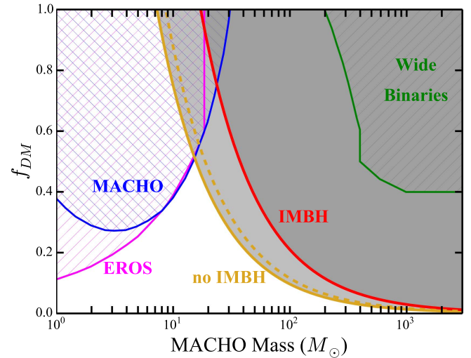
Figure 10. Constraints on MACHO dark matter following the prescription of Brandt (2016), assuming that the Eri II star cluster is located at the center of the Eri II dark matter potential. Colored curves mark exclusion regions for the maximum fraction of dark matter ( f_{\text{DM}} ) in MACHOs for a given MACHO mass. The solid yellow curve corresponds to the limits derived from the observed 3D velocity dispersion of \sigma_{3D} = 12 km s -1 and implied central dark matter density of \rho = 0.15 M_{\odot} \text{pc}^{-3} . As a comparison, the limit derived from \sigma_{3D} = 8 km s -1 and \rho = 0.02 M_{\odot} \text{pc}^{-3} from Brandt (2016) is shown as the dashed yellow curve. Since the increase in \sigma_{3D} loosens the constraint (i.e., shifts the curve rightward) and the increase in \rho strengthens the constraint (i.e., shifts the curve leftward), the combination of the two leads to similar results despite different \sigma_{3D} and \rho values. The red curve shows the MACHO constraint assuming that an intermediate-mass black hole (IMBH) with mass of 1500 M_{\odot} resides at the center of Eri II. Magenta and blue hatched contours correspond to microlensing constraints from the EROS (Tisserand et al. 2007) and MACHO (Alcock et al. 2001) experiments, respectively. The green hatched curve corresponds to constraints from the stability of wide binary stars (Quinn et al. 2009). Note that the MACHO limits from these experiments extend to much lower and higher masses than are displayed in this plot.
