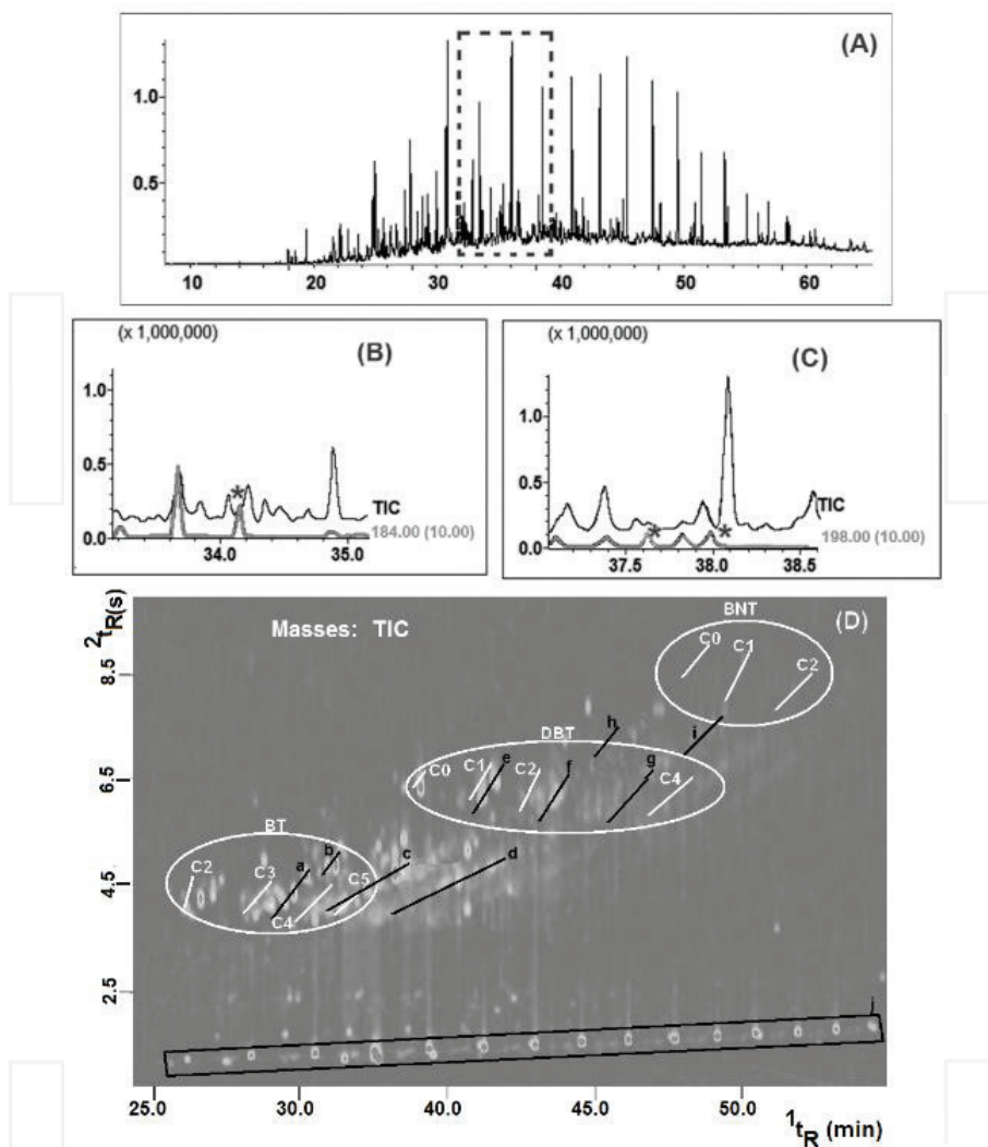
Figure 4. 1D-GC/qMS of the ASE bitumen: (A) scan mode; (B) EIM mode, with m/z 184 as the chosen ion (bellow line); (C) EIM mode, with m/z 198 as the chosen ion (bellow line). (D) GC \times GC/TOFMS color plot of ASE bitumen. White lines - sulfur compounds: benzothiophenes (BT), dibenzothiophenes (DBT), benzonaphthothiophenes (BNT); number of methyl groups attached to compounds (CX). Black lines - hydrocarbons: a, naphthalenes with three methyl groups; b, H -xanthenes; c, naphthalenes with four methyl groups; d, naphthalenes with five methyl groups; e, phenanthrenes with one methyl group; f, phenanthrenes with two methyl groups; g, phenanthrenes with three methyl groups; h, pyrenes with one methyl group; i, pyrenes with two methyl groups; j, aliphatic hydrocarbons;. (adapted from Machado et al. [99]).
