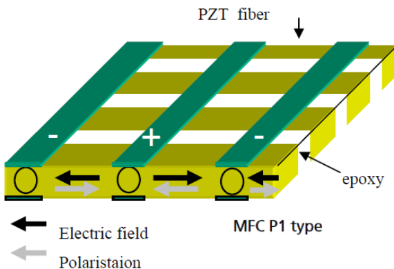
Figure 2: Electrical field and polarization for d_{33} MFC effect, Schönecker et al. (2006).
