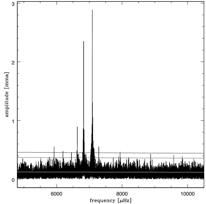
FIG. 4.—Weighted FT of the PG 0014+067 WET data expanded to the region of the most power. The mean noise level ( \sigma_{\text{noise}} ), 3 \sigma_{\text{noise}} , and 3.7 \sigma_{\text{noise}} are shown as nearly horizontal lines ( bottom to top, respectively ). [See the electronic edition of the Journal for a color version of this figure.]
