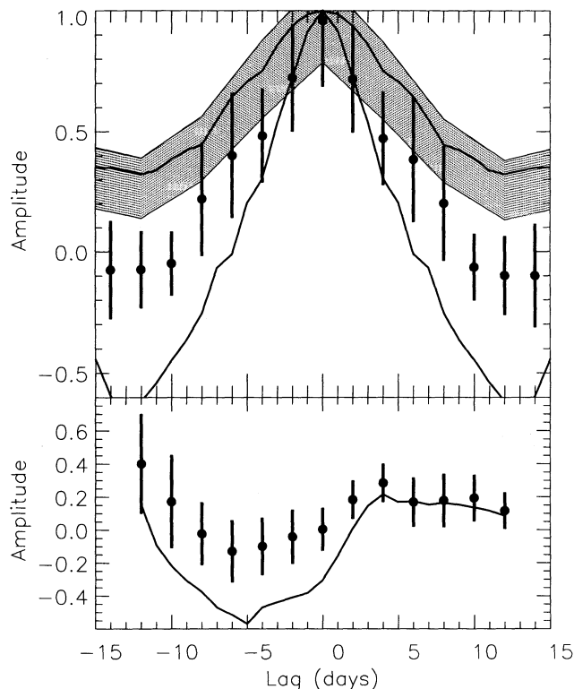
FIG. 8.—Correlations of various fluxes with the continuum flux at 1460 Å calculated for the 2 day sampling data set. All fluxes were derived from the GEX plus spectral fitting method. Top : Autocorrelation functions for the 1460 Å continuum fluxes. CCF amplitudes for the 2 day data are shown by the narrower, solid curve, corresponding DCF correlation amplitudes and uncertainties by the solid circles with error bars. The CCF and DCF autocorrelations for the 4 day sampling are also shown, as the enclosed solid curve and shaded area, respectively. The narrowness of the 2 day autocorrelations relative to those for the 4 day data, as well as the disagreement between the CCF and DCF amplitudes, reflect the presence of unresolved power on short timescales ( \lesssim 2 days) and indicate that the character of the continuum variability in NGC 3783 changed near the end of the monitoring campaign. Bottom : CCF amplitudes (solid line) and DCF amplitudes and uncertainties (circles with error bars) for the correlations of the Si III] \lambda 1892 + C III] \lambda 1909 fluxes with the continuum 1460 Å, for the 2 day sampling.
