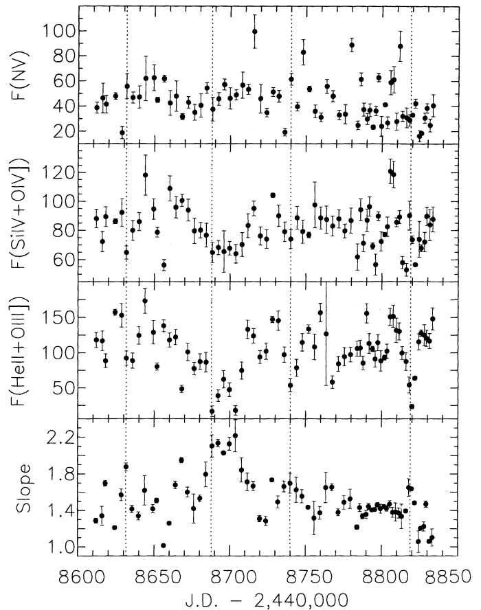
FIG. 4.—Light curves for N v \lambda 1240 (top), Si IV + O IV] \lambda 1402 (upper middle), and He II \lambda 1640 + O III] \lambda 1663 (lower middle) fluxes, and frequency spectral index \alpha_\nu (bottom). All quantities were derived from the GEX plus spectral fitting method. Fluxes are in units of 10^{-14} ergs \text{cm}^{-2} \text{s}^{-1} . Dashed vertical lines have been drawn to facilitate comparisons with Figs. 2 and 3.
