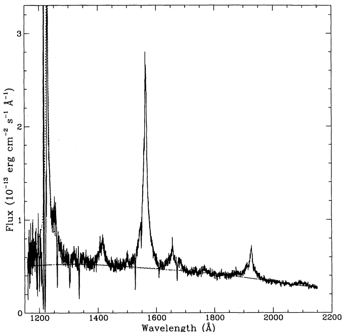
FIG. 1.—Combined FOS spectrum of NGC 3783. The underlying power-law fit to the continuum is shown as the long-dashed line. Also shown (short-dashed lines) are the sums of the components for Ly \alpha and He II, to show how these are separated from N V and O III, respectively.
