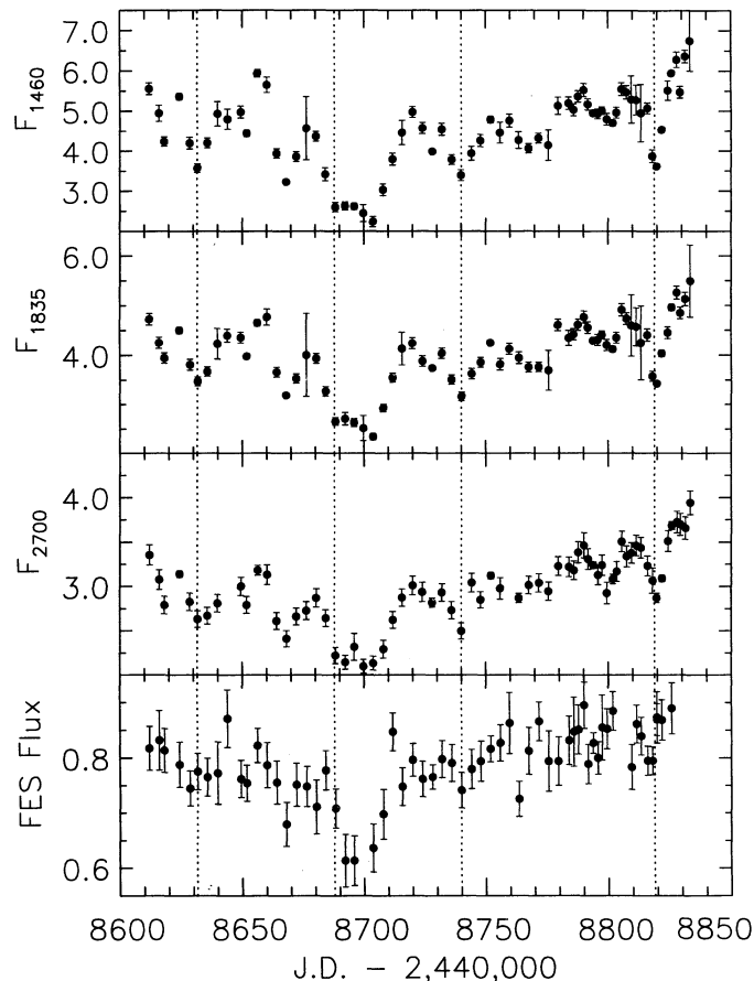
FIG. 2.—Light curves for F_{1460} (top), F_{1835} (upper middle), and relative FES fluxes (bottom). All UV fluxes are in units of 10^{14} erg \text{cm}^{-2} \text{s}^{-1} Å ^{-1} and were derived from the GEX plus spectral fitting method. The FES fluxes are as defined in eq. (3). Dashed vertical lines have been drawn to facilitate comparisons with Figs. 3 and 4.
