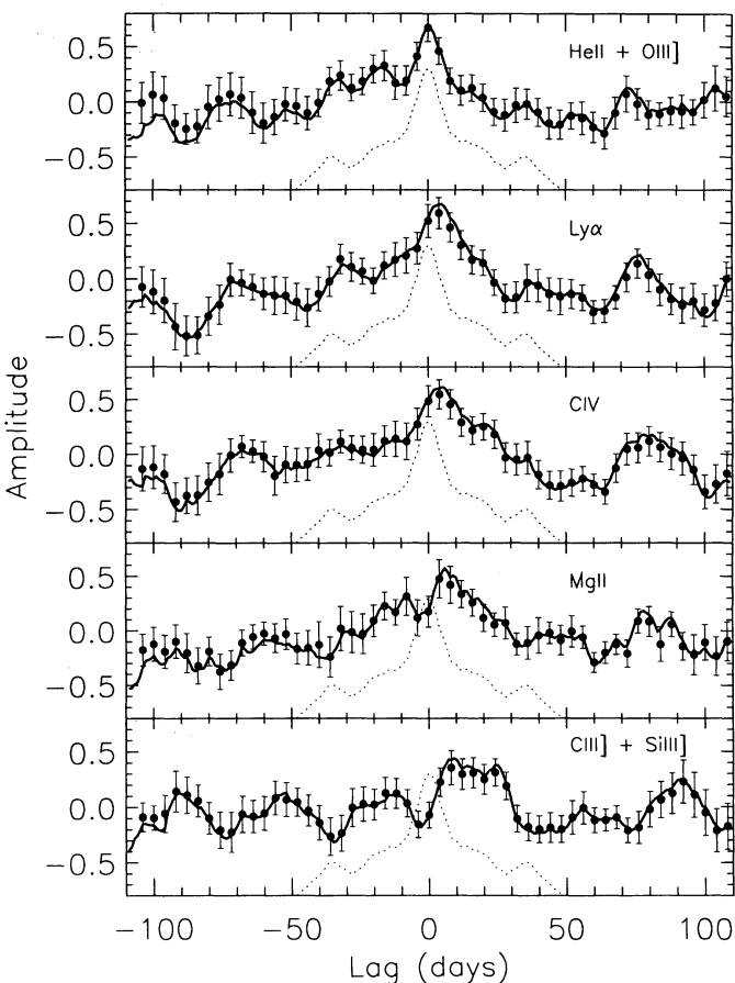
FIG. 7.—CCF and DCF correlations of various emission-line fluxes with the continuum flux at 1460 Å, based on the 4 day sampling, and calculated using the same methods as in Fig. 6. Top to bottom : CCFs and DCFs of the He II \lambda 1640 + \text{O III}] \lambda 1663 , Ly \alpha \lambda 1216 , C IV \lambda 1549 , SIPS Mg II \lambda 2798 , and Si III] \lambda 1892 + \text{C III}] \lambda 1909 emission features. The fluxes for all emission lines except Mg II were derived from the GEX plus spectral fitting method. Conventions are as in Fig. 6. The 1460 Å continuum ACF from Fig. 6 is also shown (dashed line), arbitrarily translated downward by 0.7 for clarity. Note the large values of the correlation coefficients at the peak and the very small delays of the emission lines.
