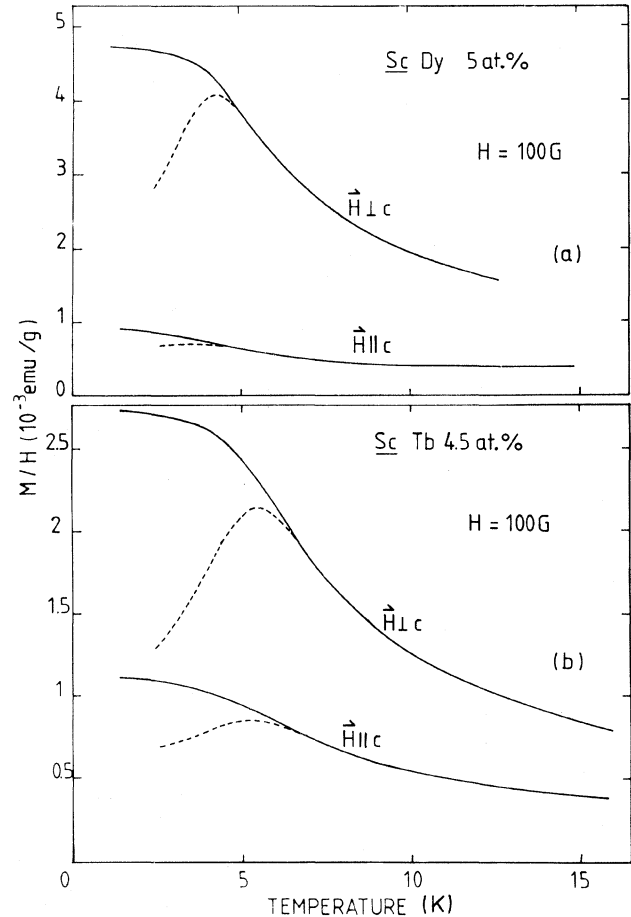
FIG. 4. ZFC (dashed line) and FC (solid line) susceptibilities of (a) ScDy 5 at.% and (b) ScTb 4.5 at.% in transverse and longitudinal fields. In both alloys and for both field directions the temperature of the maximum is lower than the temperature where the ZFC curve departs from the FC one.
