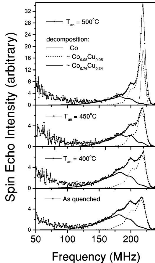
FIG. 4. Decomposition of the magnetically soft part of \text{Co}_{10}\text{Cu}_{90} melt spun ribbons. A combination of two CoCu random alloys describes the concentration modulated composition of samples annealed up to 450 °C. The alloy compositions quoted in the figure apply to the as-quenched sample—their evolution with annealing temperature is described in the text. For sample annealed at 500 °C a new line corresponding to pure Co component has to be added in the fit.
