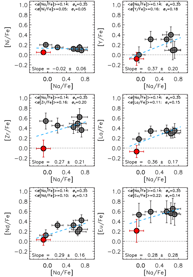
Figure 6. Same as Fig. 5 but for Ni and the neutron-capture elements versus Na.
