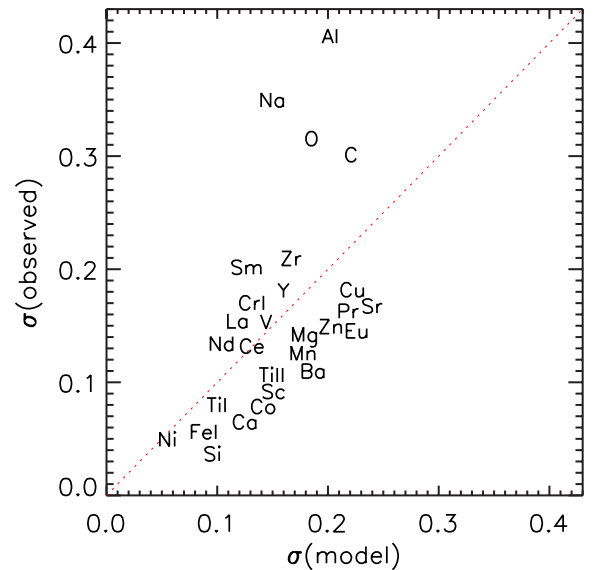
Figure 7. Measured abundance dispersion, \sigma(\text{observed}) , versus average measurement error, \sigma(\text{model}) . The dotted red line is the 1:1 relation. Fe II is not included (see text for details). For clarity, some values have been shifted by up to 0.01 dex.
